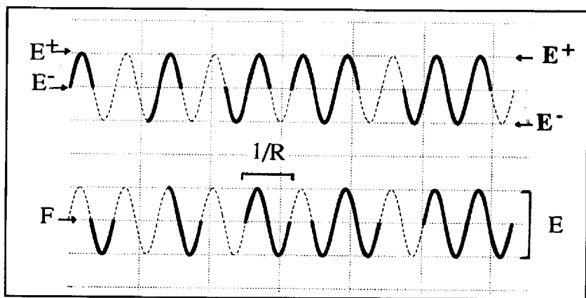
Figure 4-1. F0 patterns used in the experiments. E: vibrato extent; F: vibrato nominal frequency; R vibrato rate; E+: F0 maximum; E-: F0 minimum
