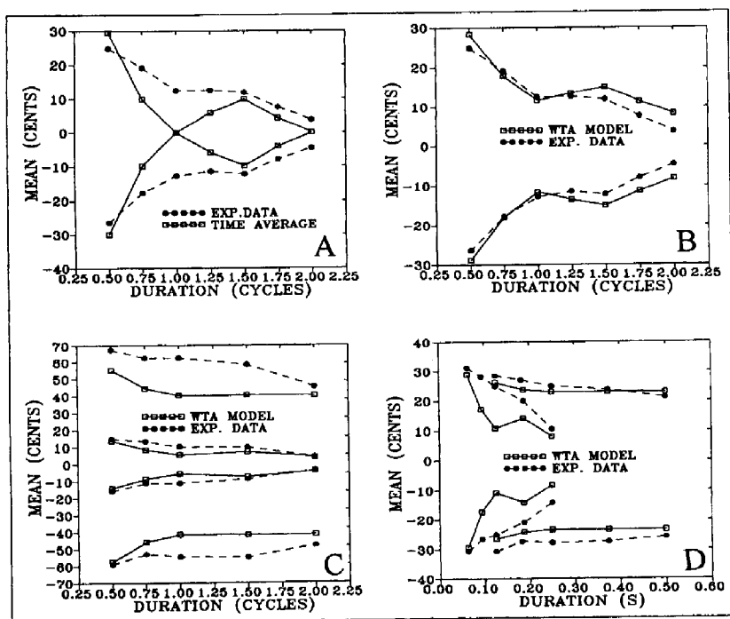
Figure 4-4. Models. A: time-average, main experiment. B: WTA, main experiment. C: WTA, P1; D: WTA P3
