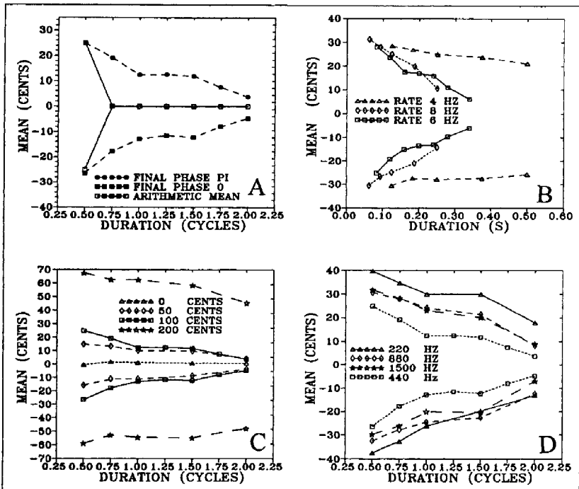
Figure 4-2. Experimental data. A: main experiment and mean frequency model; B: P3; C: P1; D: P2
